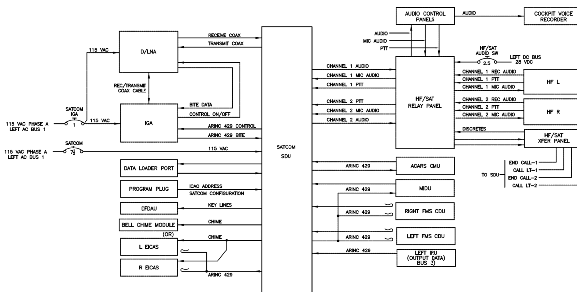
FIGURE 4: SATCOM System Block Diagram
