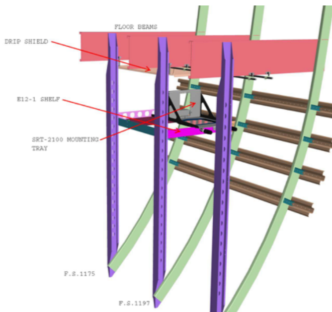
FIGURE 2: E12-1 Shelf Installation
