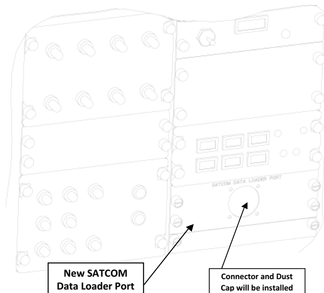
FIGURE 3: SATCOM Data Loader Port Installation
