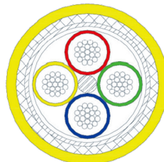
100 Base-T Shielded Quad
