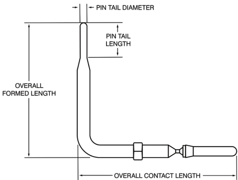
PC Right-Angle Contact
